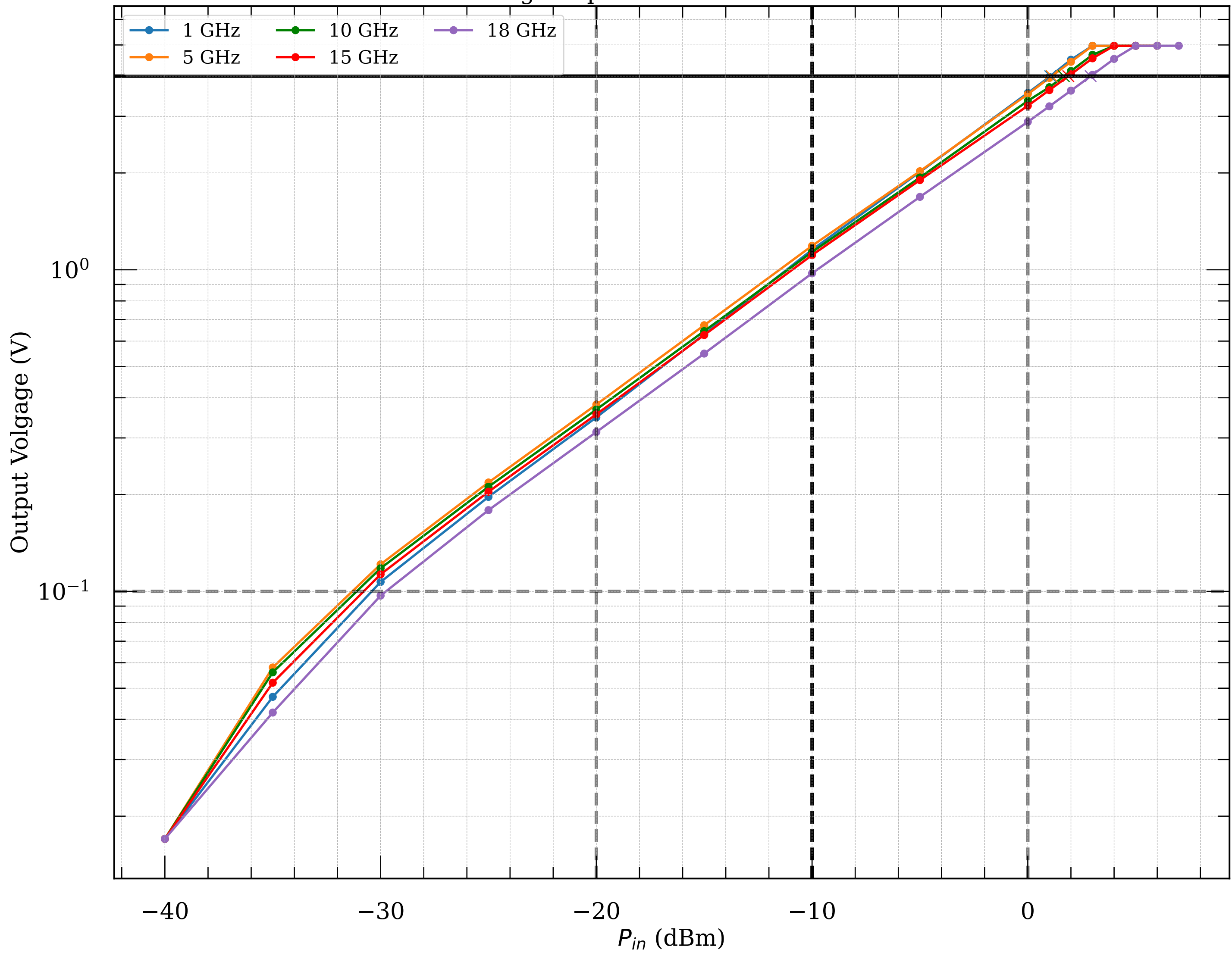
Measured voltage-to-power curve of detector module078
